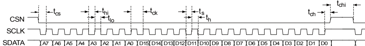
Figure 3. Serial Port Interface timing
