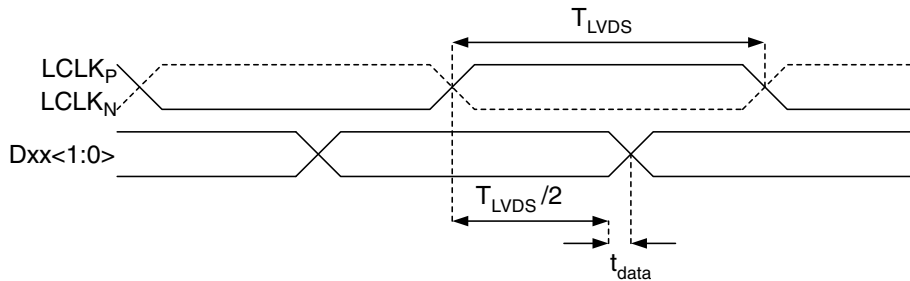
Figure 7. LVDS data timing, DDR mode
